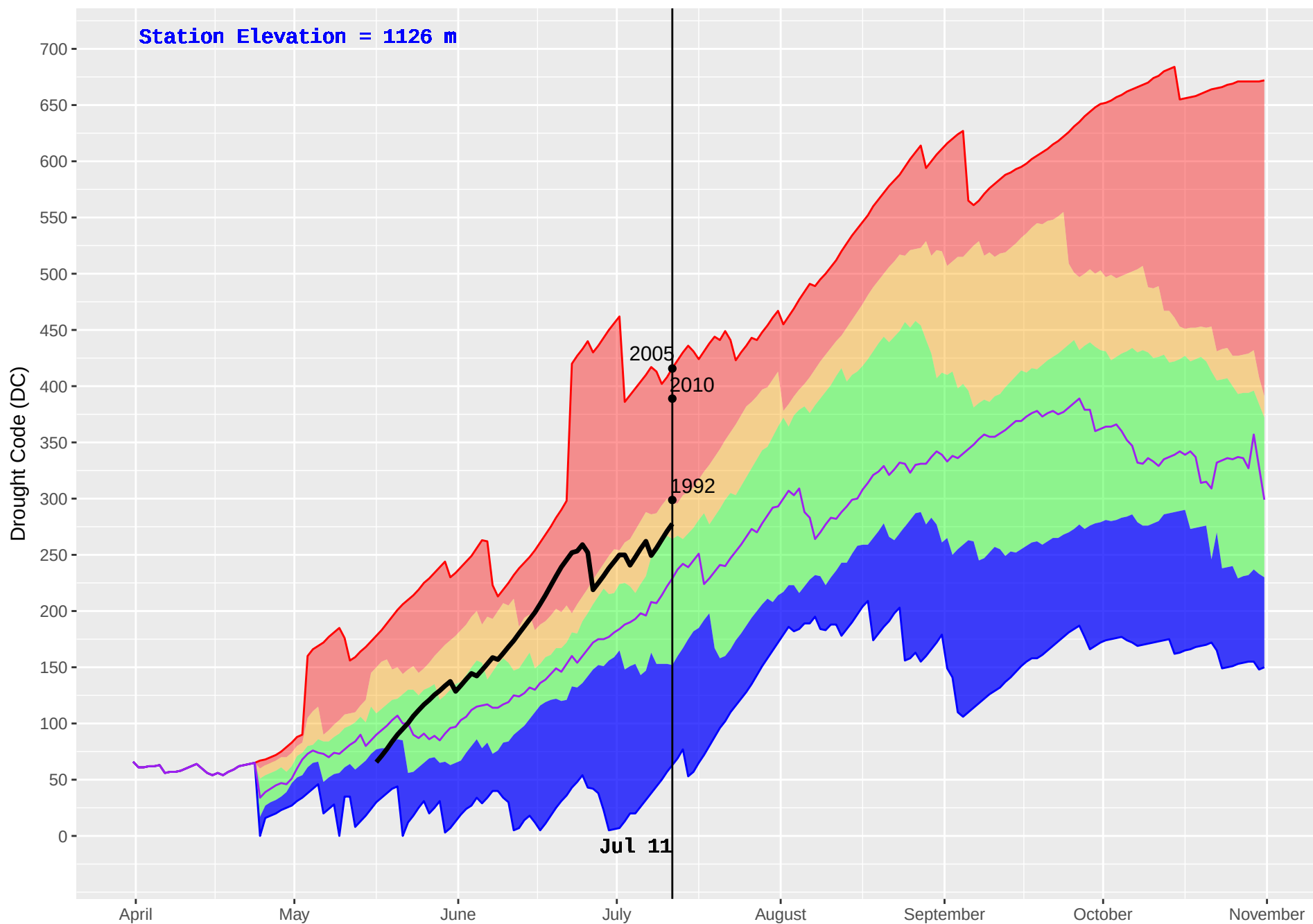
BLACKPINE (148) : Historical (1980–2016) and Current (2018) Noon Drought Code (DC)
