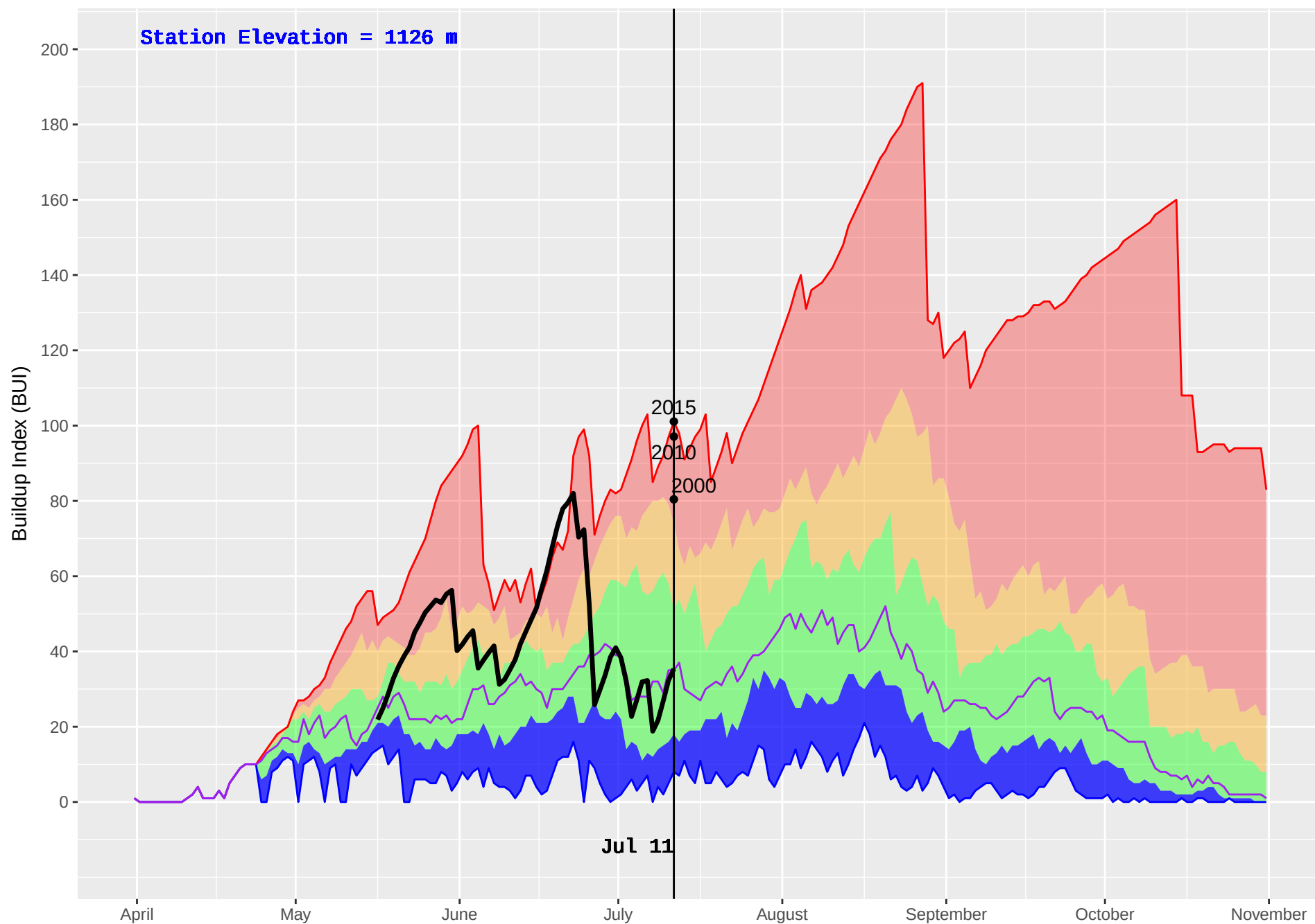
BLACKPINE (148) : Historical (1980–2016) and Current (2018) Noon Buildup Index (BUI)
