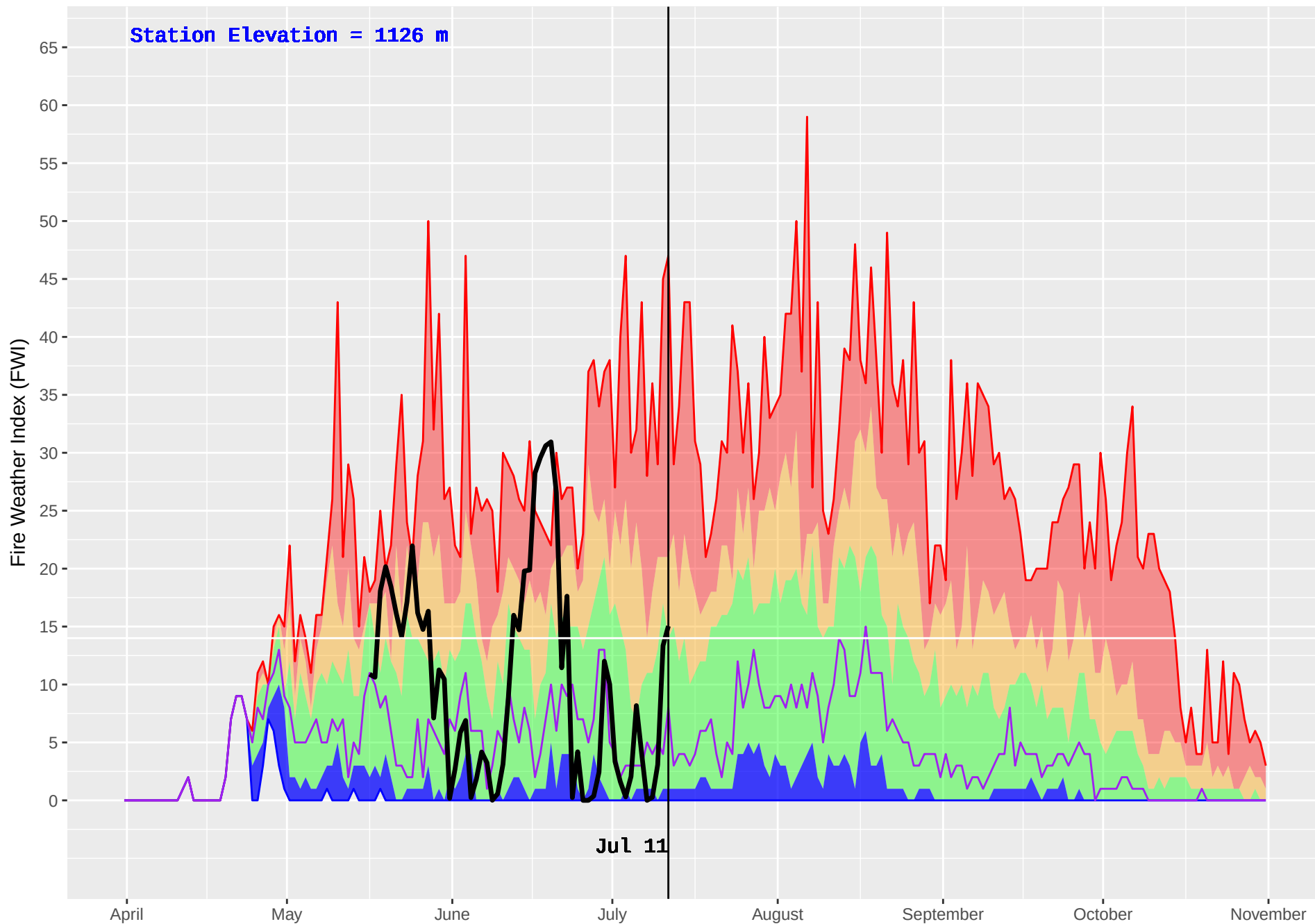
BLACKPINE (148) : Historical (1980–2016) and Current (2018) Noon Fire Weather Index (FWI)
