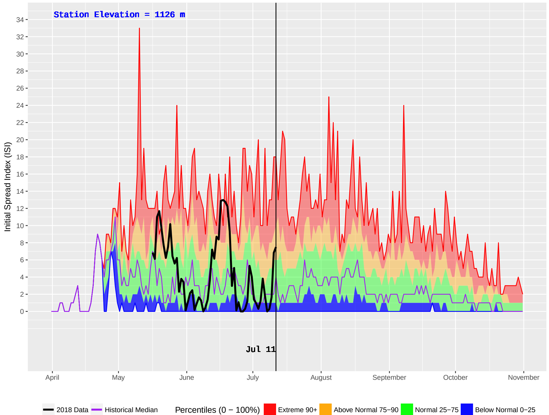
BLACKPINE (148) : Historical (1980–2016) and Current (2018) Noon Initial Spread Index (ISI)
